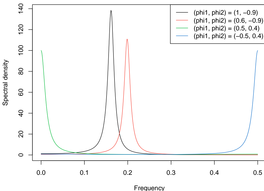
Figure 7: Spectral density for the second-order AR model, for a few parameter choices \phi_1, \phi_2 .
